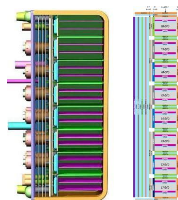
The HCLL Test Blanket Module (left) and MELCOR model (right)
