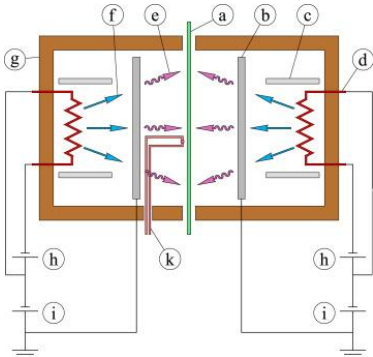
< Schematic cross-section of the sample heating system
