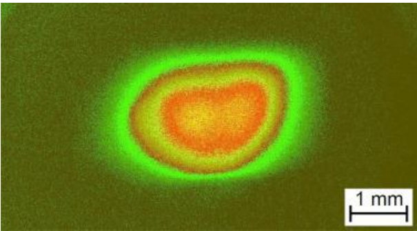
False-color image of the ion current density on the ITO-coated glass >
